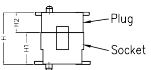
Mating Section
